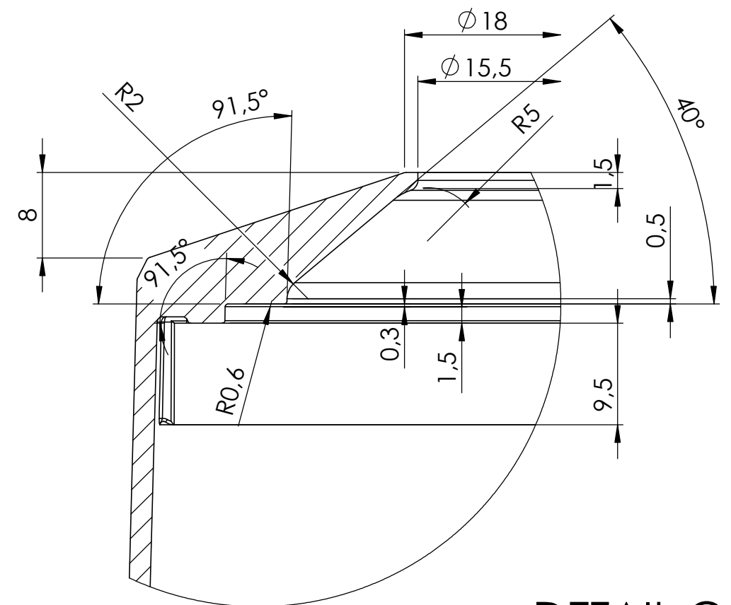
DETAIL C SCALE 2 : 1
